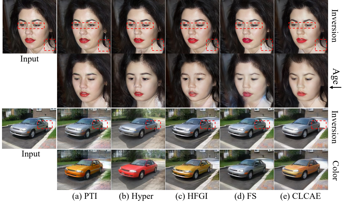
Figure 5. Visual comparison of inversion and editing between our method and the baseline methods (PTI [53], Hyper [6], HFGI [59], and FS [63]) in the \mathcal{F} group. We produce \text{CLCAE} = G(w^+, f) to compare with them. Our method not only generates high-fidelity reconstruction results but also retains the flexible manipulation ability. \downarrow means a reduction of the manipulation attribute.
