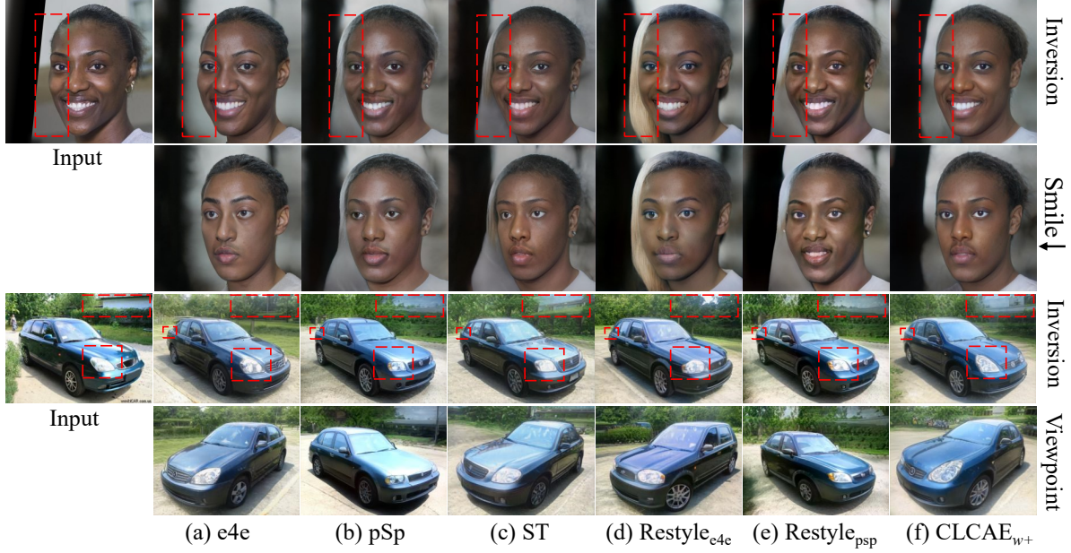
Figure 4. Visual comparison of inversion and editing between our method and the baseline methods (e4e [56], pSp [52], ST [25], restyle e4e [5] and restyle pSp [5]) in the \mathcal{W}^+ group. We produce \text{CLCAE}_{w^+} = G(w^+) to compare with them. Our method is more effective in producing manipulation attribute relevant and visually realistic results. ↓ means a reduction of the manipulation attribute.
