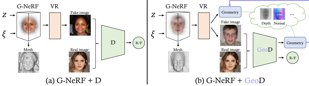
Figure 1: Concept comparison between (a) existing 3D-aware GANs where only the generator is made 3D-aware with the help of NeRF [19], and (b) our GeoD where the discriminator supervises the generator with the extracted geometry. Such an additional task ( i.e. , geometry extraction) substantially improved 3D-aware GANs with more accurate 3D shapes (see meshes). Here, z and \xi denote a sampled latent code and camera pose, respectively, while “VR” stands for volume rendering [19].
