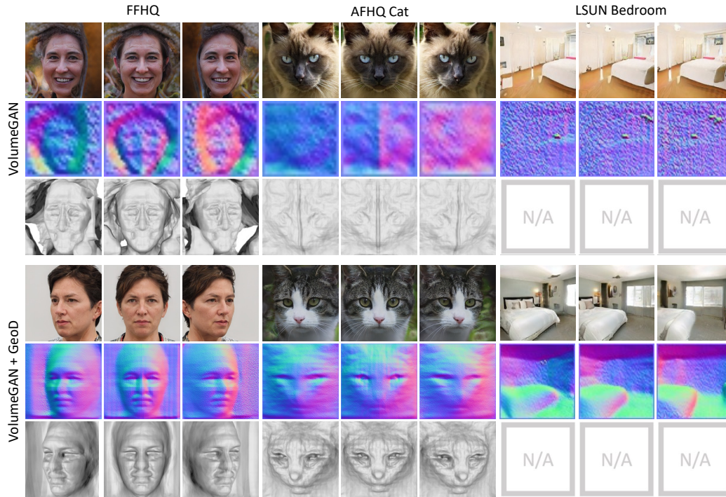
Figure A6: Qualitative results with VolumeGAN [34] as the base model. From top to bottom: synthesized results, normal maps derived from the generative neural radiance field, and 3D meshes.
