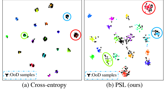
Figure 5. Feature representation visualization of cross-entropy and our PSL method. OoD samples are in black and InD samples are in other colors. In the red, blue and green circles, it is clear that OoD samples distribute at the edge of InD samples in our PSL, while greatly overlap with each other in the cross-entropy method.
