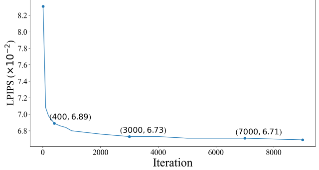
Figure 7. Our model with different optimization iterations.
