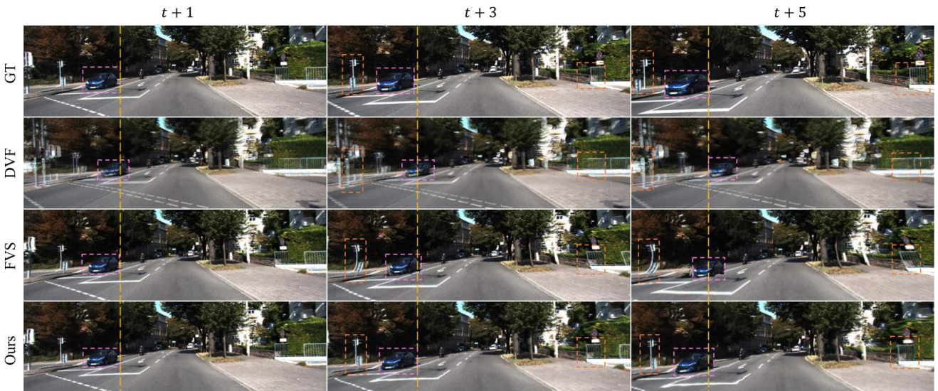
Figure 3. Multi-frame prediction comparison on KITTI. As the pink boxes show, DVF [20] fails to separate the motion of the blue car from the background and produces a “zooming-in” effect, which is the major motion exhibited in the dataset, caused by the forward movement of the running car. FVS [45] wrongly predicts the motion of the blue car at t + 3 and t + 5 , resulting in incorrect frame prediction results. Our model can correctly capture the motion of the blue car without external training.
