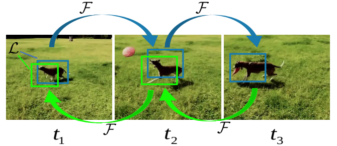
Fig. 1. Illustration of our self-supervised cycle-consistent framework. Given the bounding box (in blue) of the target object in the first frame, the object is tracked forward (in blue) in subsequent frames and then circularly tracked backward (in green) to the first frame. The discrepancy between the initial bounding box and the predicted box in the first frame can be used to serve as the supervision to optimize the tracking network \mathcal{F}(\mathbf{z}, \mathbf{x}; \theta) .
